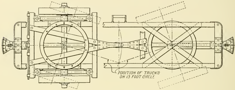
Fig. 5. Plan of Schiemann Trailer
